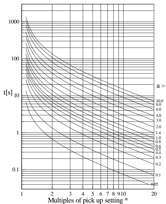
Figure 5.6: Very Inverse
