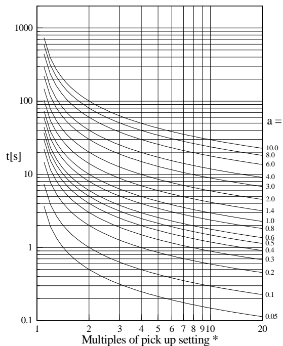
Figure 5.5: Normal Inverse
